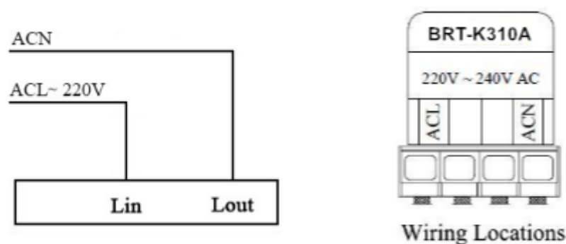
Fig. 3 BRT-K310A Wiring Diagram
