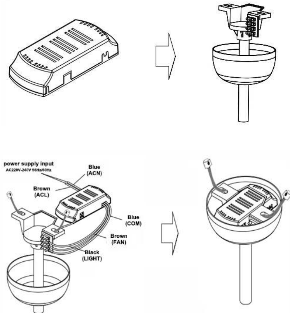
Fig. 4 AS-CF236T Receiver Installation
