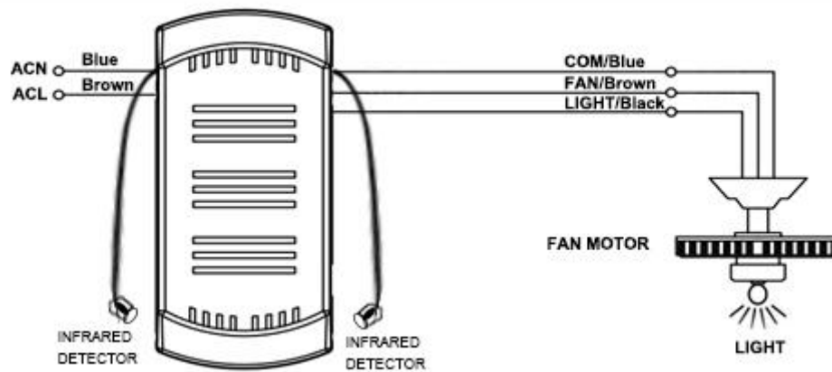
Fig. 3 AS-CF236L Receiver Wiring Diagram
