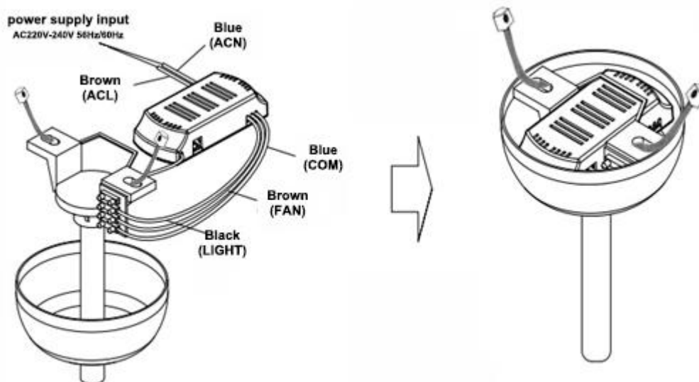
Fig. 4 AS-CF236L Receiver Installation
