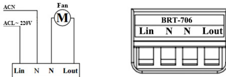
Fig. 3 BRT-706 Wiring Diagram
