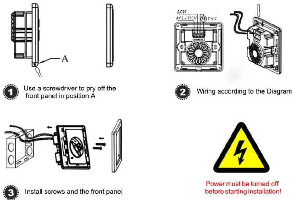
Fig. 4 BRT-706 Installation Guide
