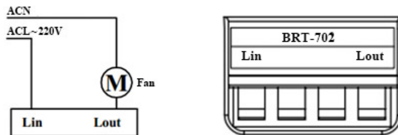
Fig. 3 BRT-702 Wiring Diagram
