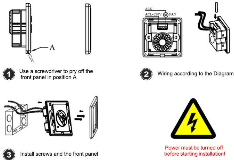
Fig. 4 BRT-702 Installation Guide
