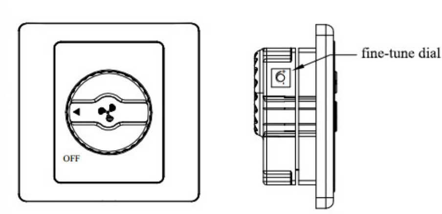
Fig. 5 Adjust the Minimum Speed
