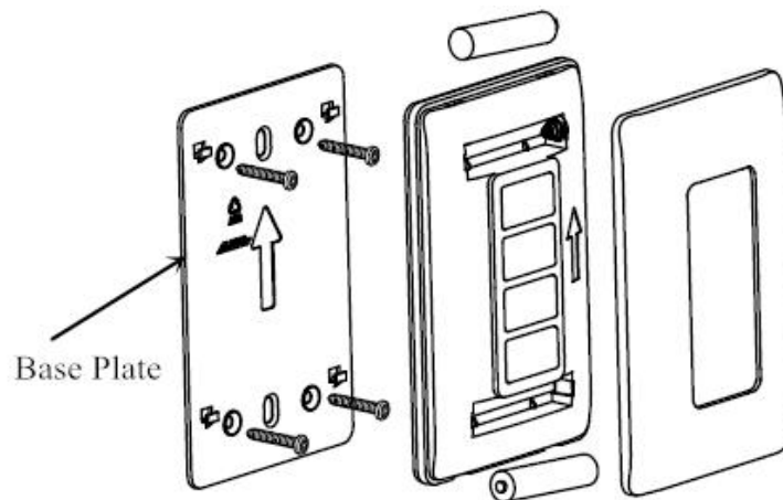
Fig. 6 Installation of BRT-690M
