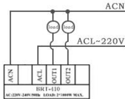
Fig. 4 Wiring Diagram of Wall Mount Unit
