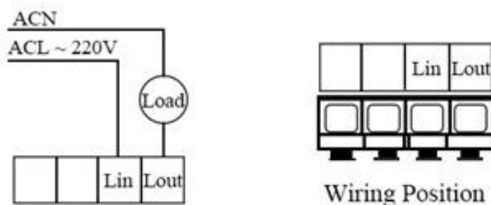
Fig. 4 Wiring Diagram of Wall Mount Unit
