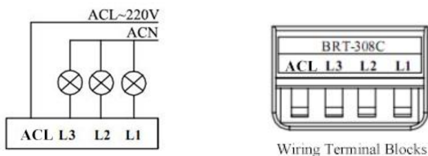
Fig. 3 BRT-308 Wiring Diagram
